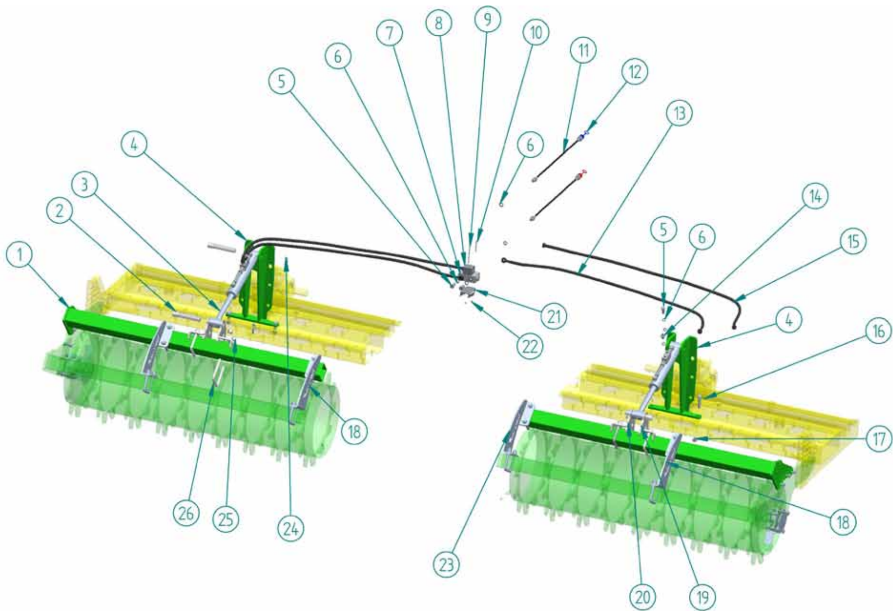
RULLO REGOLABILE EKOS - HYDRAULIC ADJUSTABLE ROLLER EKOS
