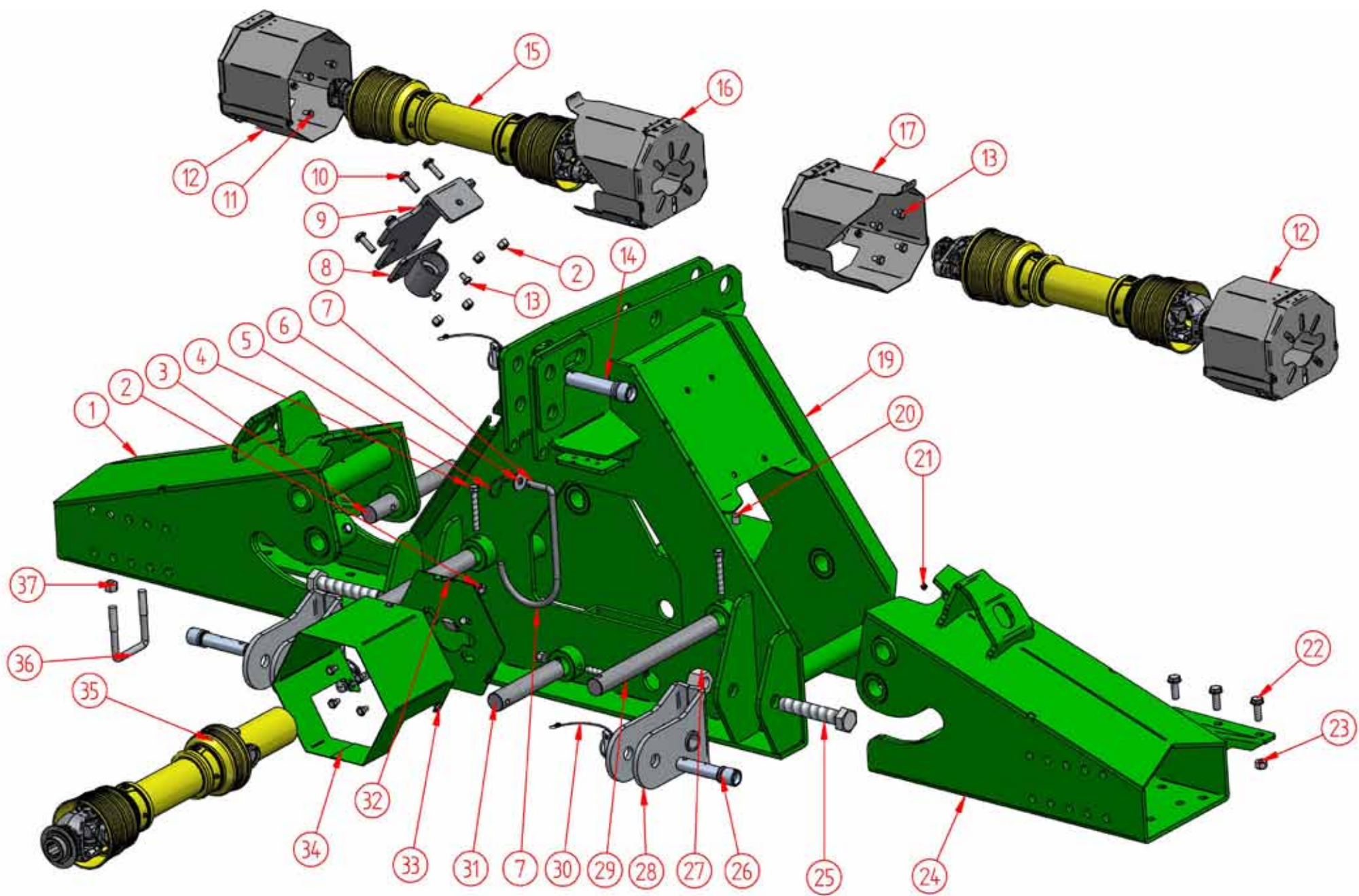
EKOS- EKOS THIRD POINT LINKAGE
